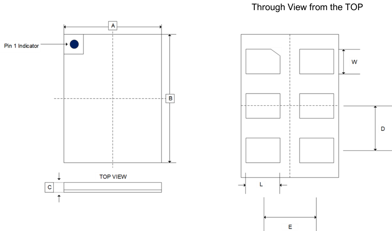
Figure 20. MS1133 Packaging Drawing (2.5X2.0 mm)
