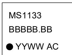
Figure 24. MS1133 Device Top Marking Showing Pin 1
