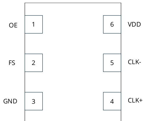
Figure 2. MS1133/MS1183 Pin Assignments
