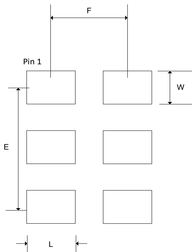
Figure 23. MS1183 Packaging Land Pattern Drawing (2.0X1.6 mm)
