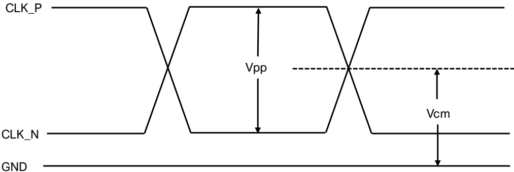
Figure 16. HCSL Output Level across differential pair (CLK_P-CLK_N)
