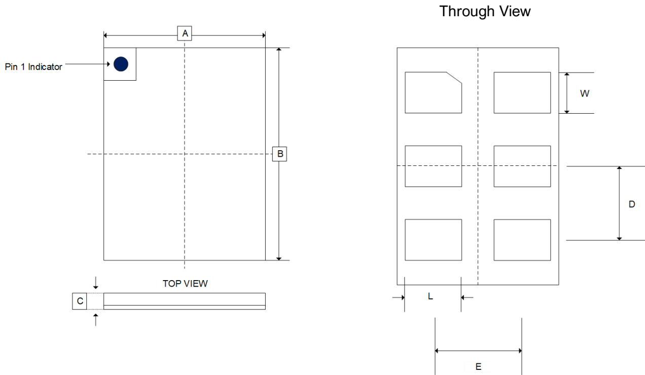
Figure 19. MS1150 Packaging Drawing (2.5X2.0 mm)
