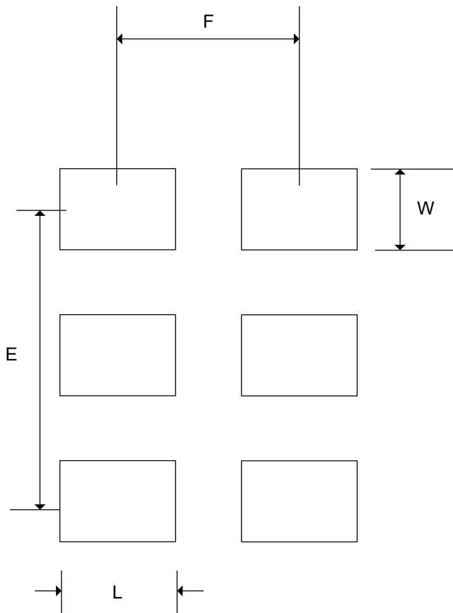
Figure 20. MS1150 Packaging Land Pattern Drawing (2.5X2.0 mm)
