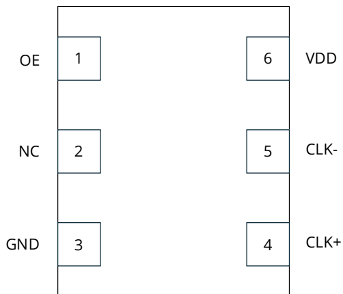
Figure 2. MS1150 Pin Assignments
